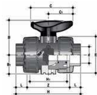
VKDIV/SHX 2-way ball valve with handle lock and STAINLESS steel threaded inserts with female ends for solvent welding, metric series
