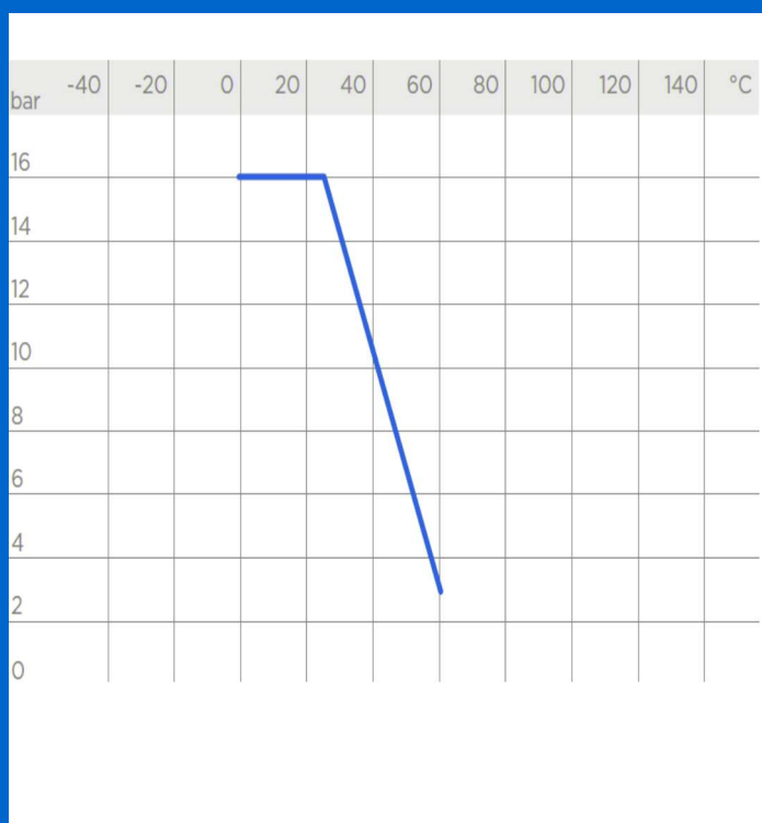
VKDIV 2-way ball valve with female ends for solvent welding, metric series
